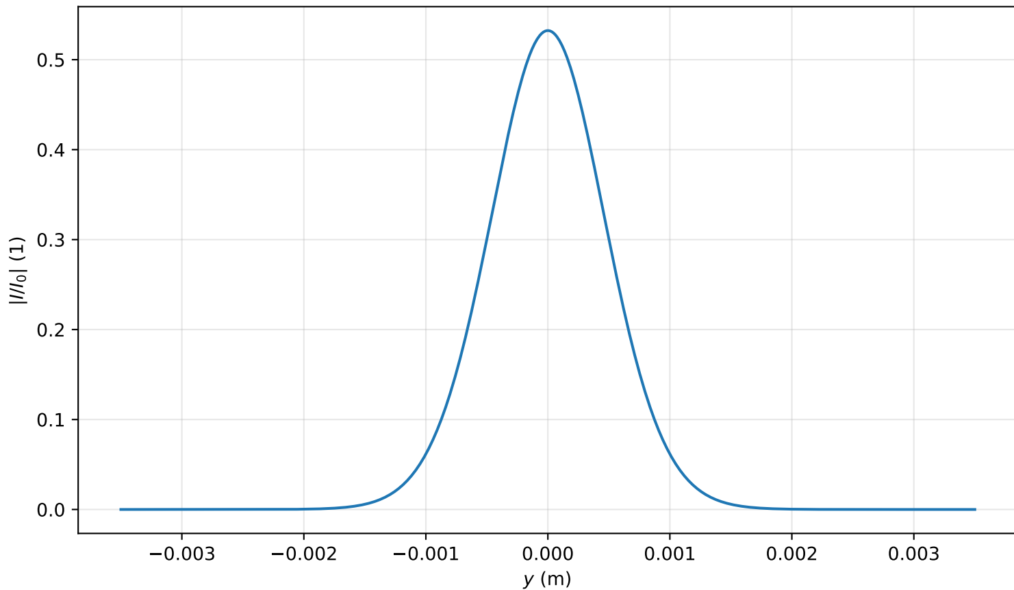
Intensity profile I(x=0, y, z=2.229)/I_0 , P_{in}=0.2P_{cr} , artificial time
